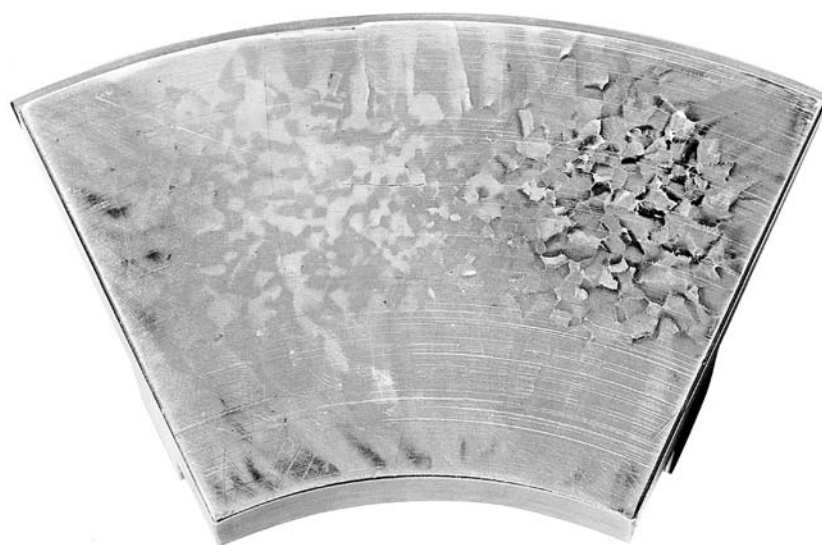
Figure 4. Thermal Ratcheting
