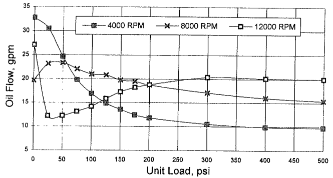
Figure 12. Standard LEG Oil Flowrate for Fixed Pressure Test.
