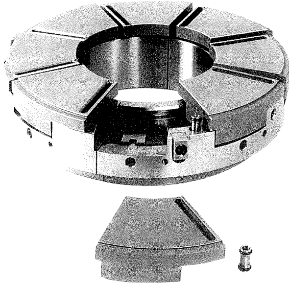
Figure 2. Test LEG Thrust Bearing.
