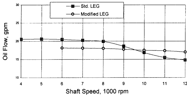
Figure 22. Oil Flowrate Versus Speed at 50 PSI Unit Load for Fixed Valve Test for the Modified LEG and Standard LEG.
