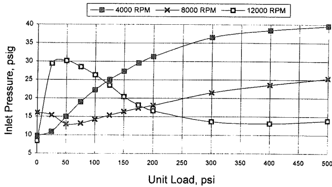
Figure 9. Standard LEG Oil Supply Pressure for Fixed Valve Test.
