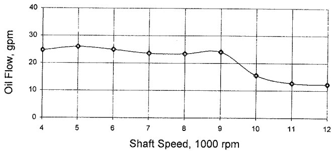
Figure 10. Standard LEG Oil Flowrate Versus Speed for Fixed Pressure Test at 50 PSI Unit Load.
