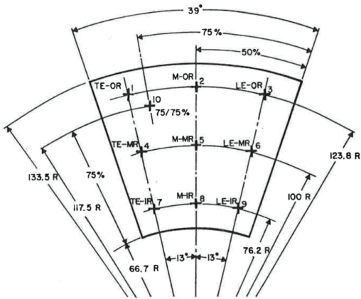
Fig. 1-Location of bearing pad thermocouples in the babbitt
