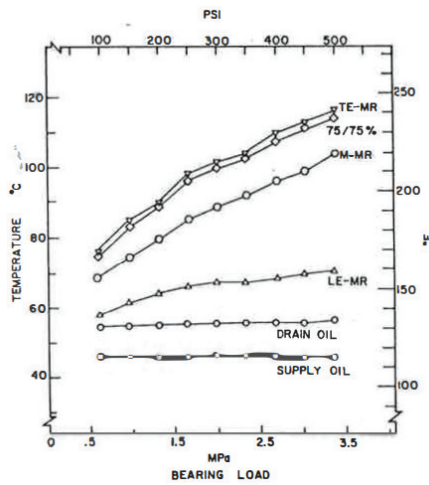
Fig. 7—Same as Fig. 5 except 150 percent recommended flows, are almost exactly identical to curves in Fig. 7, which represents the same temperature data collected during tests run with 150 percent of the recommended flows.
