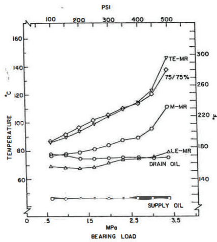
Fig. 10 - Same as Fig. 4 except 10,000 rpm 50 percent produced parallel shifts of the drain oil temperature curves up or down, depending on whether the amount of oil was increased or decreased. This is attributed to only the slight influence that oil film temperature has on bulk oil temperature (5).
