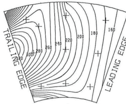
Fig. 2 — Bearing Pad Isotherm Showing the thermal gradient across the pad at a shaft speed of 10,000 rpm and a load of 3.45 MPa (500 psi) with 100 percent of recommended flow rate. Temperatures shown are in °F.
