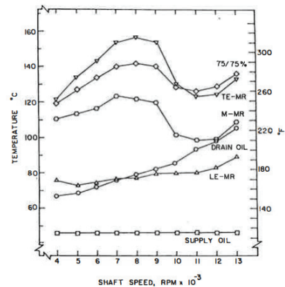
Fig. 6 — A comparison of the temperatures recorded at selected locations for a bearing operating at a load of 3.45 MPa, for shaft speeds that ranged from 4,000 to 13,000 rpm, using a lubricant supplied at 50 percent of recommended flow rates at a temperature of 46°C.
