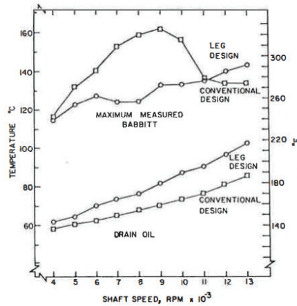
Fig. 11 - A comparison of maximum measured babbitt temperatures and drain oil temperatures of conventional and leading-edge-groove bearings operating at a load of 3.45 MPa, for shaft speeds ranging from 4,000 to 13,000 rpm, using an ISO VG 32 lubricant supplied at 46°C.
