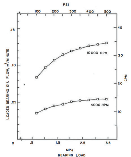
Fig. 9 — A comparison of the 4,000 and 10,000 rpm shaft speed 100 percent recommended oil flow rates to the loaded bearing, for loads that range from 0 to 3.45 MPa, using an ISO VG 32 lubricant supplied at 46°C.
