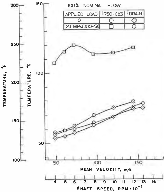
Fig. 9 Effect of shaft speed and load on pad babbltt temperatures—304-mm (12-in.) bearing
