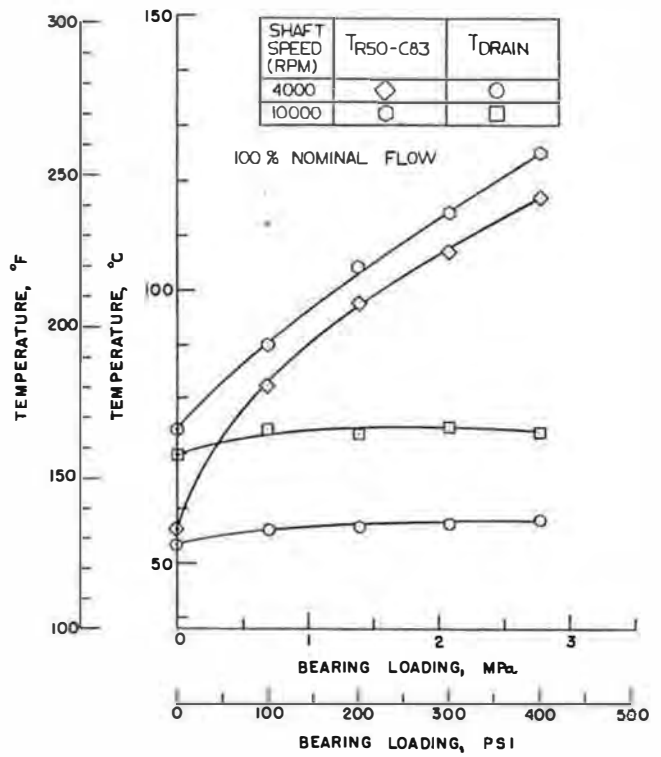
Fig. 10 Effect of load and shaft speed on pad babbltt temperatures—304-mm (12-in.) bearing
