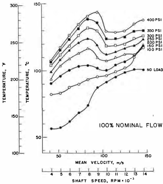
Fig. 8 267-mm thrust bearing maximum babbltt temperatures at pad locallon 4 ( T_{R50-C83} )
