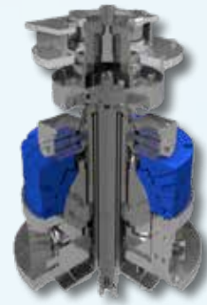
Cutaway of test rig showing Kingsbury spherical tilt pad bearing in blue
